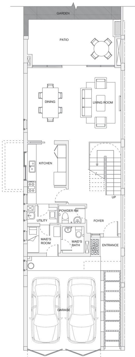
GROUND FLOOR PLAN WITH CLOSE KITCHEN
