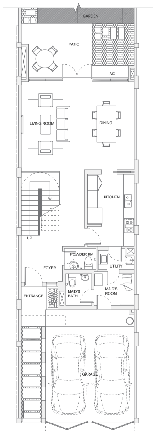
GROUND FLOOR PLAN WITH CLOSE KITCHEN
