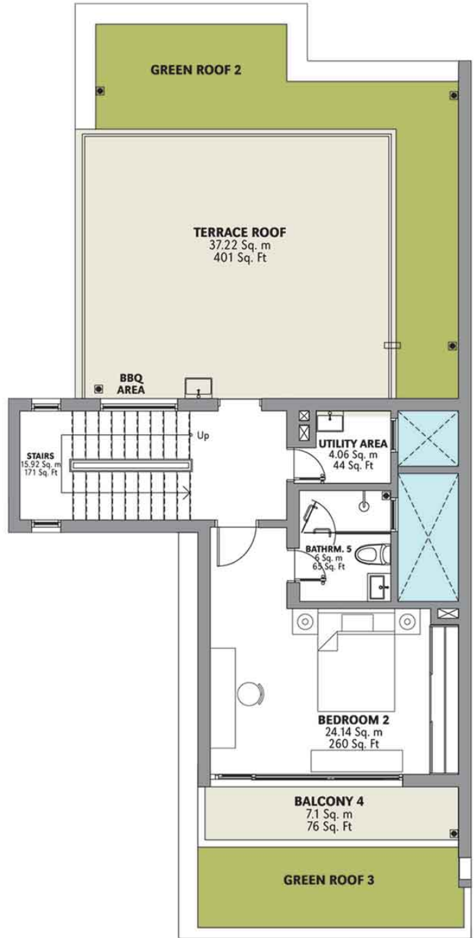
THIRD FLOOR
