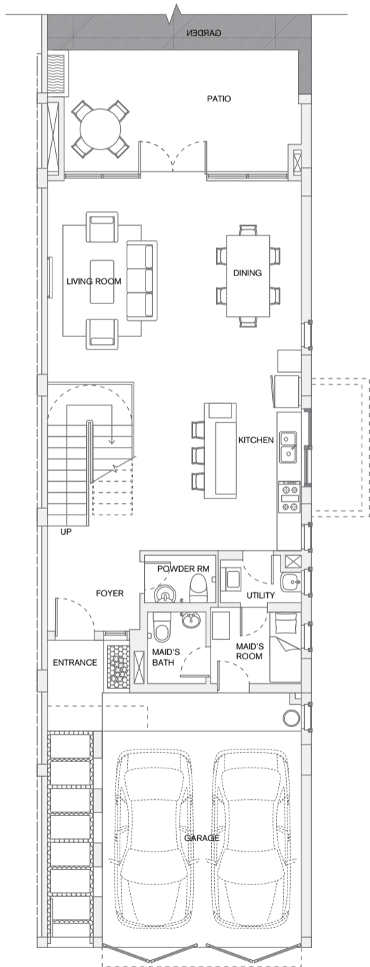
GROUND FLOOR PLAN WITH OPEN KITCHEN
